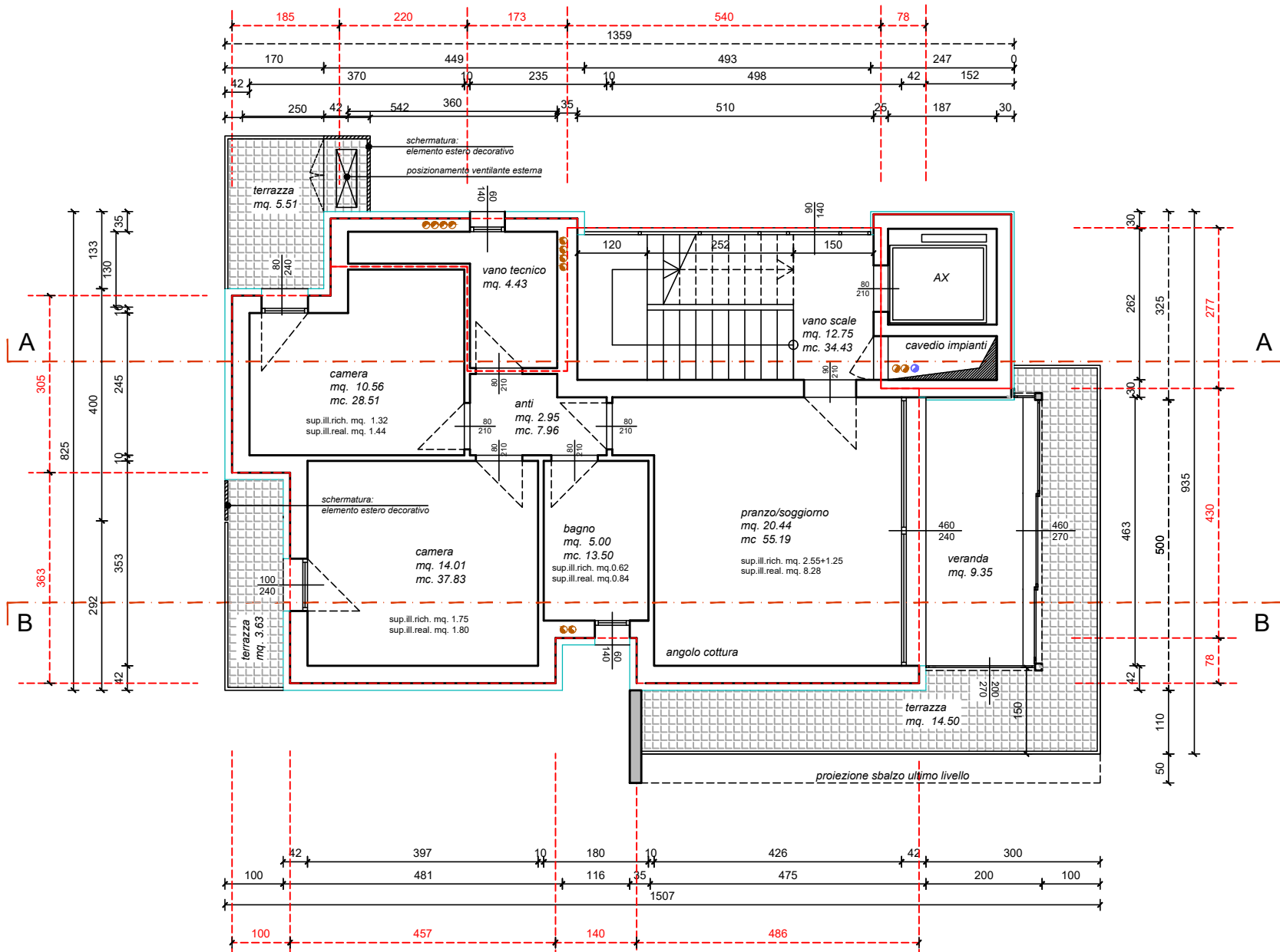
PIANTA PIANO 2-3-4-5-6
